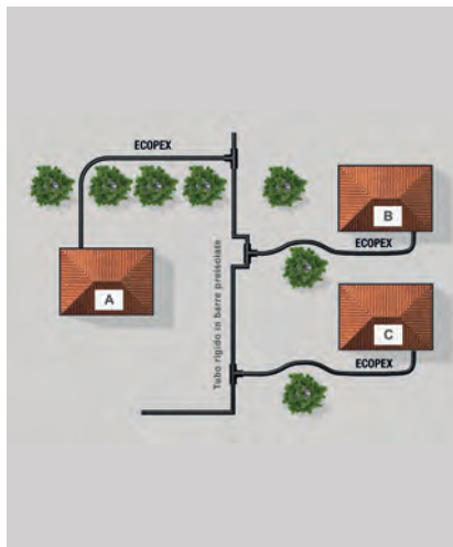
BRANCH FROM RIGID PREINSULATED NETWORK BUILDING TO BUILDING CONNECTION
